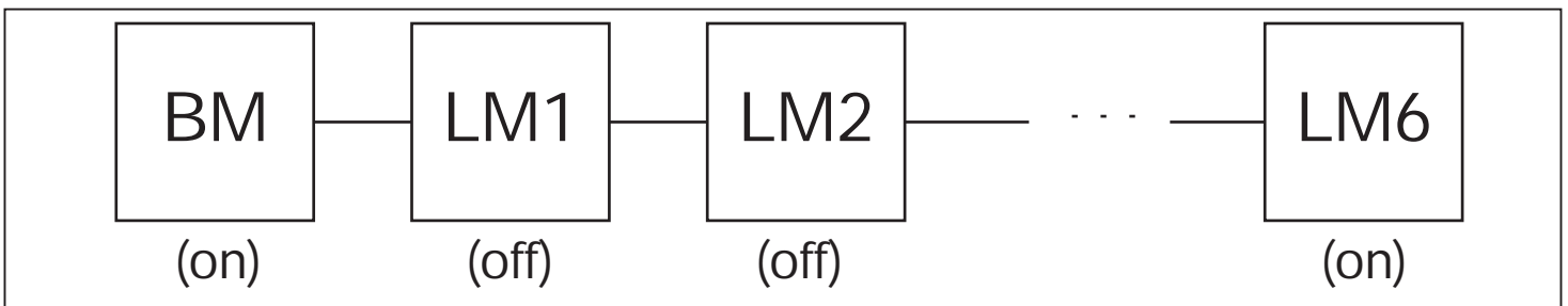
BM ... Basic module ES5403 (or else compact wall scanner ES5400) LM1 – LM6 ... Scanner module 1 to scanner module 6
